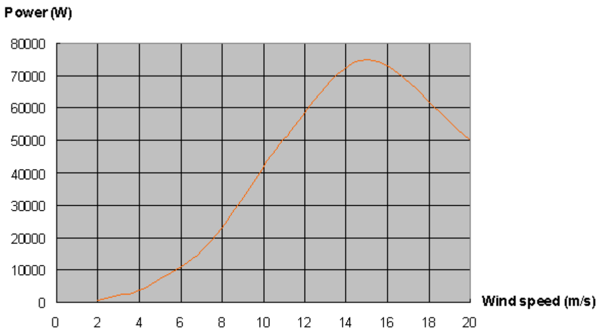
HUMMER-50KW Wind Generator
